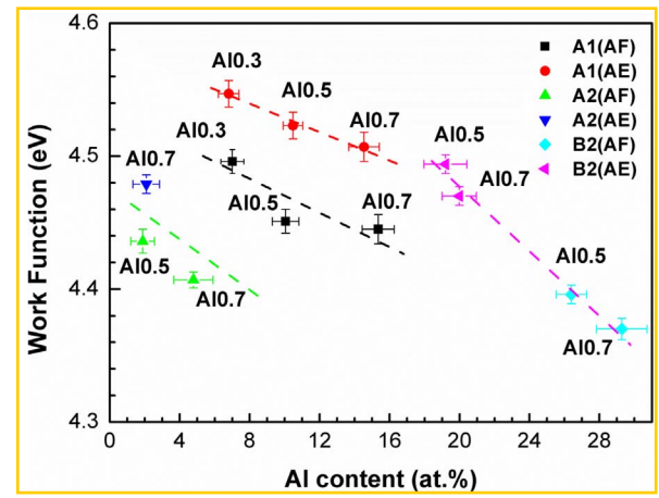
Fig. 10. Changing trends of work functions for A1 (disordered FCC), A2 (disordered BCC) and B2 (ordered BCC) phases in \text{Al}_{0.3}\text{CoCrFeNi} ( \text{Al}_{0.3} ), \text{Al}_{0.5}\text{CoCrFeNi} ( \text{Al}_{0.5} ) and \text{Al}_{0.7}\text{CoCrFeNi} ( \text{Al}_{0.7} ) HEAs of as-forged (AF) and as-equilibrated (AE) conditions, as a function of Al content.
