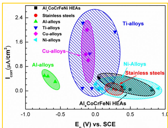
Fig. 11. Comparison of corrosion properties between HEAs and conventional alloys [60–66] in the 3.5 wt.% NaCl solution. The higher pitting potential ( E_p ) and lower corrosion-current density ( I_{\text{corr}} ) of Al x CoCrFeNi HEAs indicate that the localized and general corrosion-resistant properties of the Al x CoCrFeNi HEAs are comparable or even superior to that of conventional corrosion-resistant alloys.
