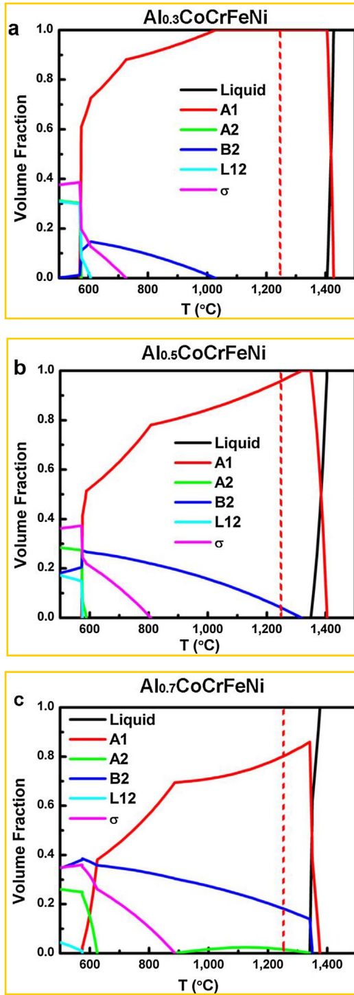
Fig. 9. Equilibrium calculations of phase fractions as a function of temperature for the \text{Al}_x\text{CoCrFeNi} ( x = 0.3, 0.5 and 0.7 ) alloys. (a) \text{Al}_{0.3}\text{CoCrFeNi} , (b) \text{Al}_{0.5}\text{CoCrFeNi} , and (c) \text{Al}_{0.7}\text{CoCrFeNi} . The red-dash-lines are located at the temperature of 1250^\circ\text{C} .
