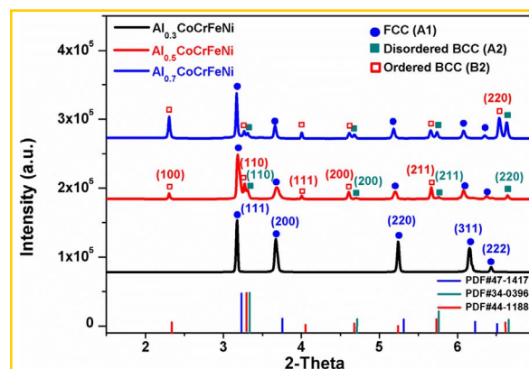
Fig. 1. High-energy X-ray diffraction pattern of the Al 0.3 CoCrFeNi ( x = 0.3, 0.5 and 0.7 ) alloys.
