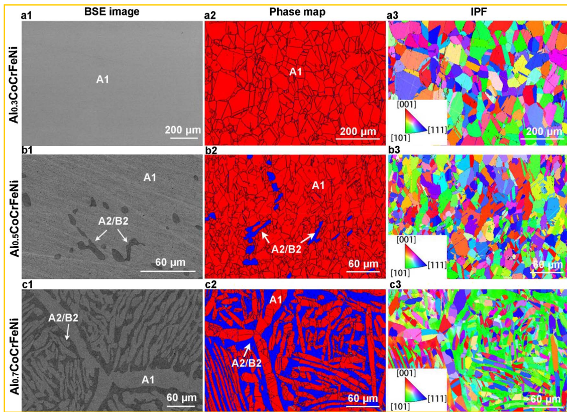
Fig. 2. Microstructures of the as-forged \text{Al}_x\text{CoCrFeNi} ( x = 0.3, 0.5 and 0.7 ) alloys. (a1–c3) are the backscattered electron (BSE) image, phase map, and inverse pole-figure (IPF) of the as-forged \text{Al}_{0.3}\text{CoCrFeNi} (a1–a3), \text{Al}_{0.5}\text{CoCrFeNi} (b1–b3), and \text{Al}_{0.7}\text{CoCrFeNi} (c1–c3), respectively.
