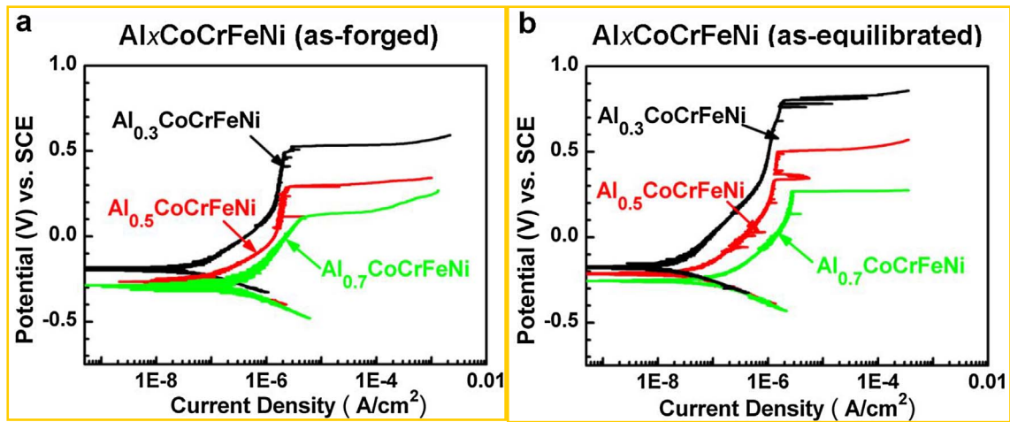
Fig. 7. Potentiodynamic polarization curves of the as-forged (a) and as-equilibrated (b) \text{Al}_x\text{CoCrFeNi} ( x = 0.3, 0.5 and 0.7 ) alloys, performed with the scan rate of 100 mV/min in the 3.5 wt.% NaCl solution at room temperature.
